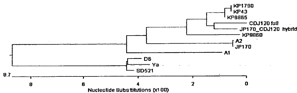
Phylogenetic tree
